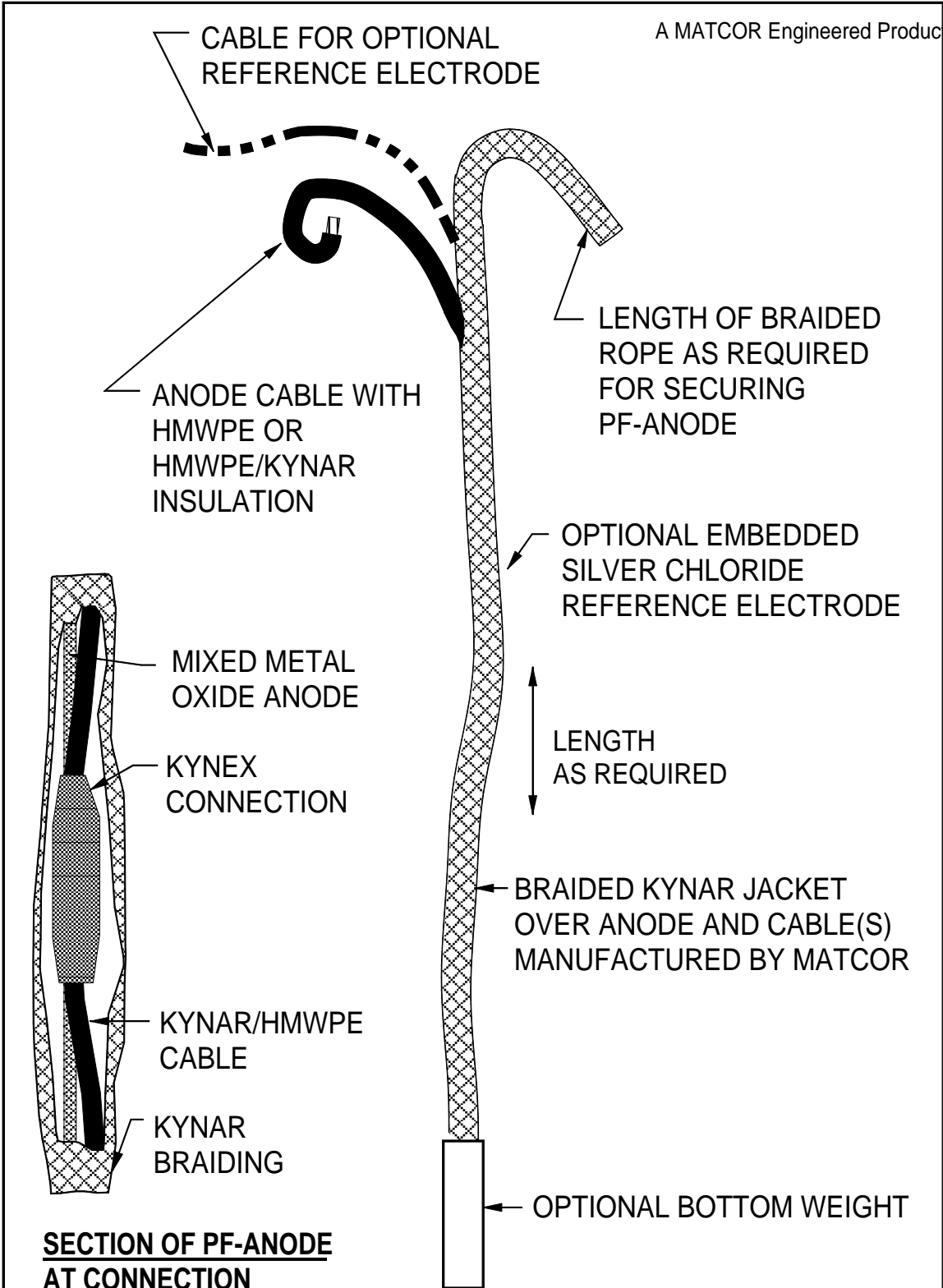
COMPLETE ANODE ASSEMBLY
