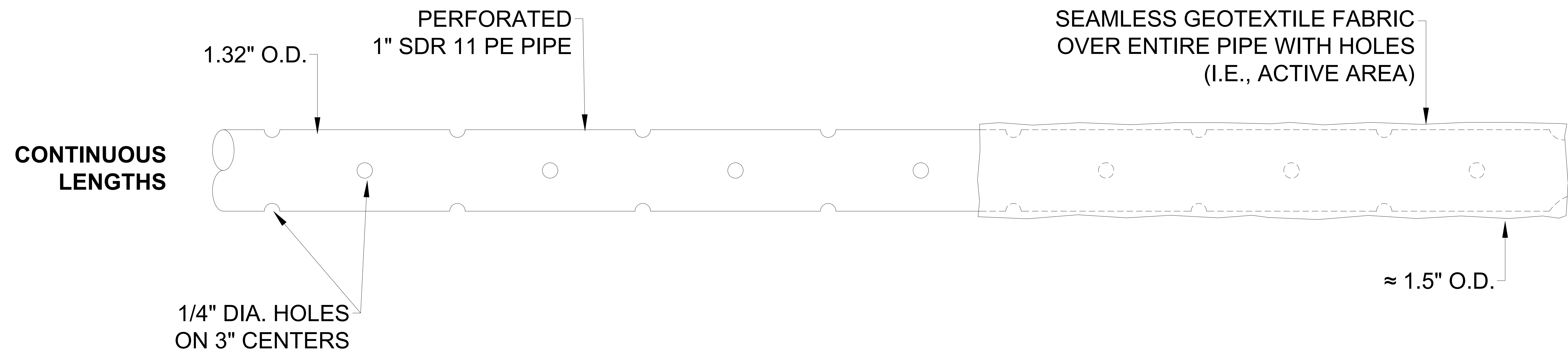
1 SUPERVENT™ DEEP ANODE VENT PIPE
